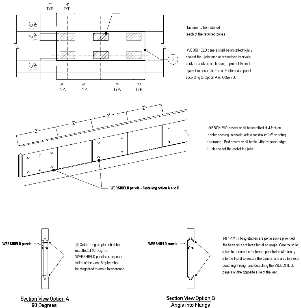
FIGURE 8 – WEBSHIELD® INSTALLATION DETAILS (3x2 Flange)
