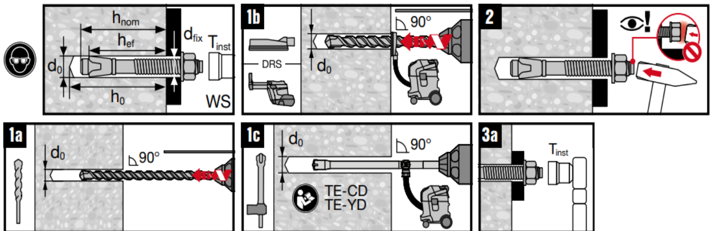
FIGURE 5 – MANUFACTURER’S PUBLISHED INSTALLATION INSTRUCTIONS (MPII)
