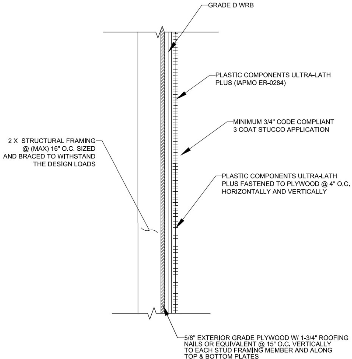
FIGURE 1 - Assembly (Continued on next two pages)
