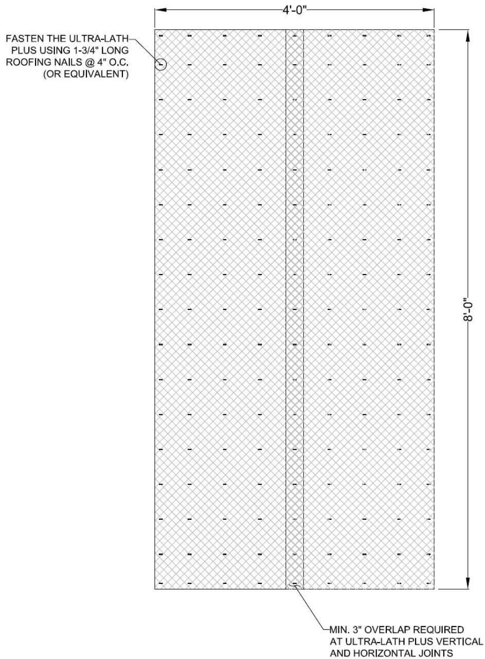
FIGURE 1 - Assembly (Continued)
