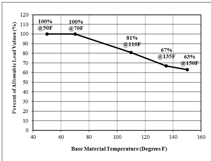
FIGURE 1—LOAD CAPACITY BASED ON IN-SERVICE TEMPERATURE FOR SET-XP® EPOXY ADHESIVE
