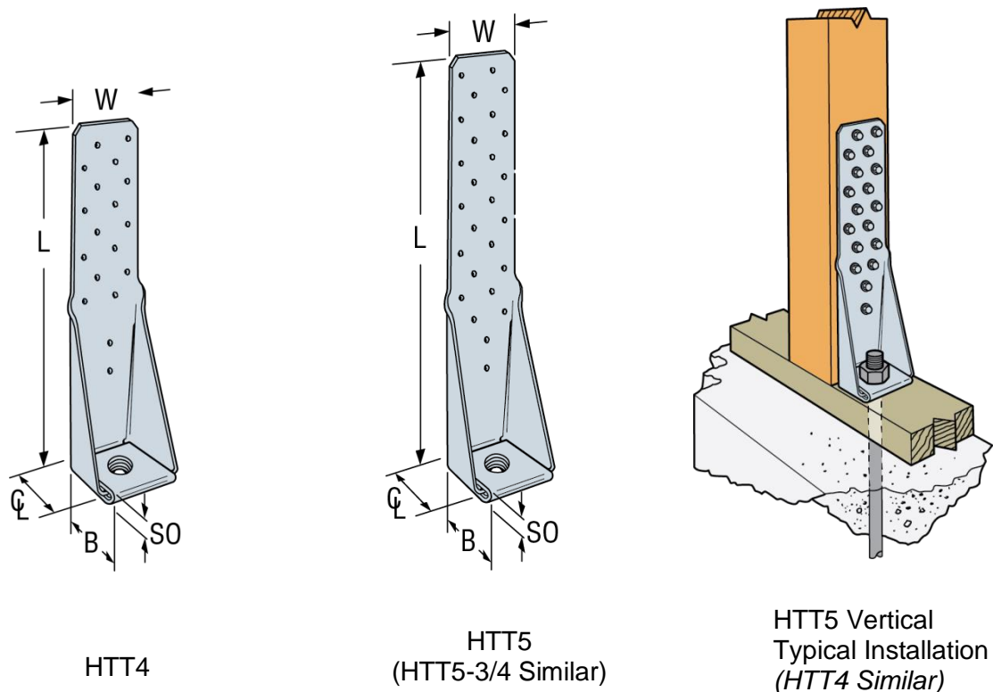
Figure 2 – HTT Nail Hold-Downs
