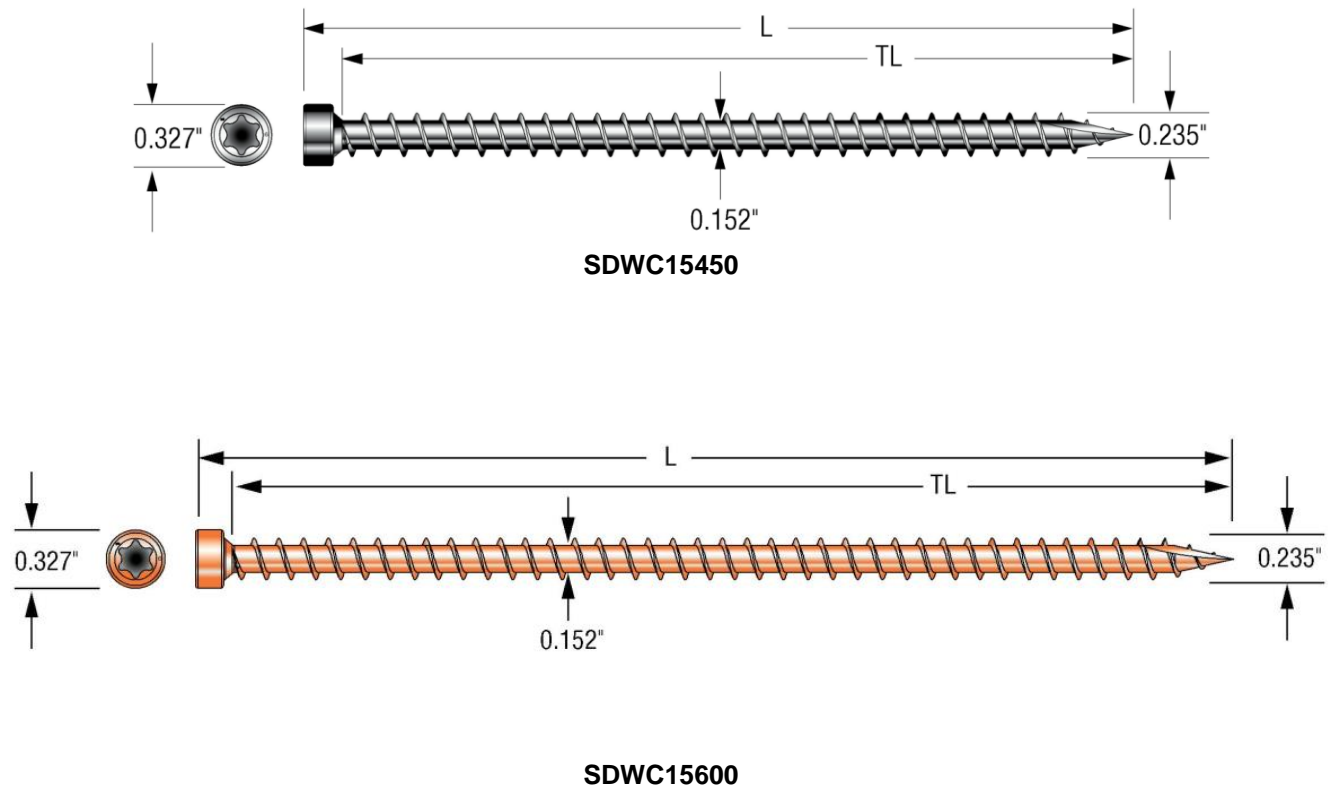
FIGURE 1 – SDWC SCREWS
