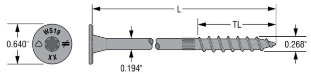
FIGURE 4 – SDWS19 SCREWS
