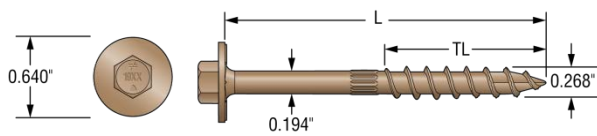
FIGURE 3 – SDWH19DB SCREWS
